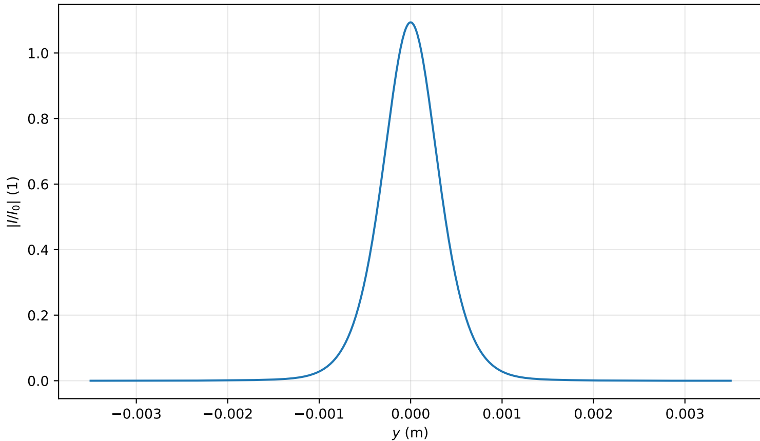
Intensity profile I(x=0, y, z=3.025)/I_0 , P_{in}=0.8P_{cr} , artificial time
